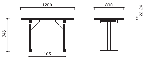
Standard Folding Table 4680-27
